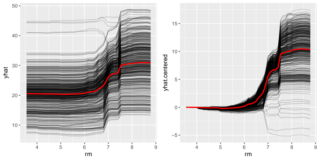
Figure 10: ICE curves (black curves) and their average (red curve) depicting the relationship between medv and rm for the Boston housing example. Left: Uncentered (here the red curve is just the traditional PDP). Right: Centered.
