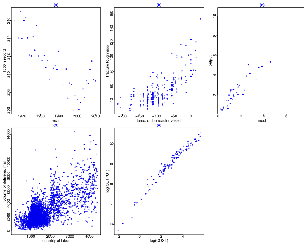
Figure 1: From left to right and from top to bottom, the scatterplots of the yearly best men's outdoor 1500-metre run times in seconds, the 254 nuclear reactors' data, the 37 European Air Controllers, the 4000 European post offices and the 123 American electric utility companies.
