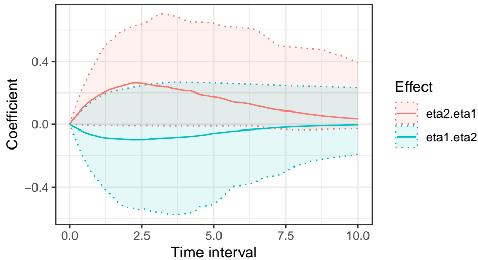
Figure 2: Discrete-time cross-effect dynamics of the estimated system for a range of time intervals, with 95% credible intervals.
