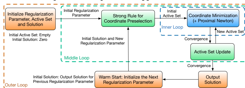
Figure 1: The pathwise coordinate optimization framework with 3 nested loops: (1) Warm start initialization; (2) Active set selection, and strong rule for coordinate preselection; (3) Active coordinate minimization.
