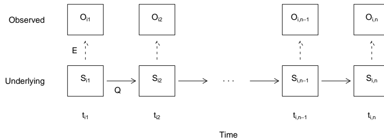
Figure 9: A hidden Markov model in continuous time. Observed states are generated conditionally on an underlying Markov process.
