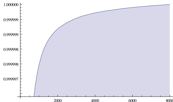
Figure 1: Runtime distribution in (4, 4). More than 99.9999% of the Turing machines that stopped in 8000 steps or less actually halted before 2000 steps.
