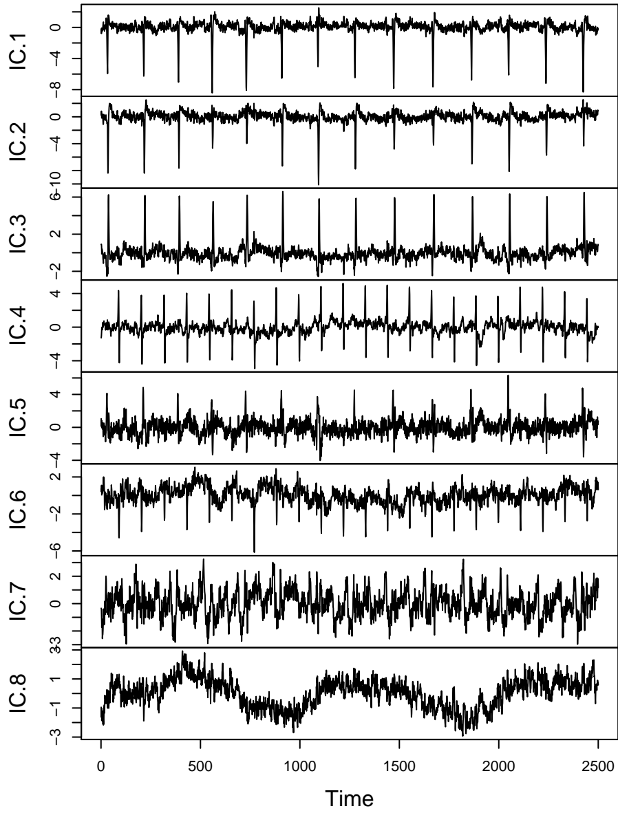
Figure 5: The independent components estimated with the JADE method.
