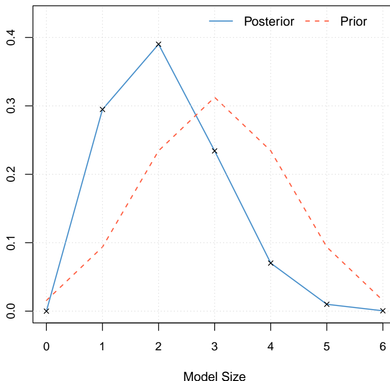
Posterior Model Size Distribution Mean: 2.1121
